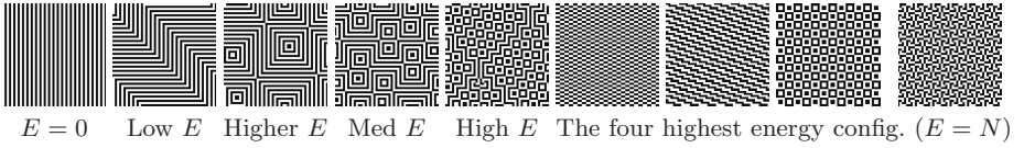
Fig. 6. Examples of stable configurations for 2D Minority at various levels of energy
