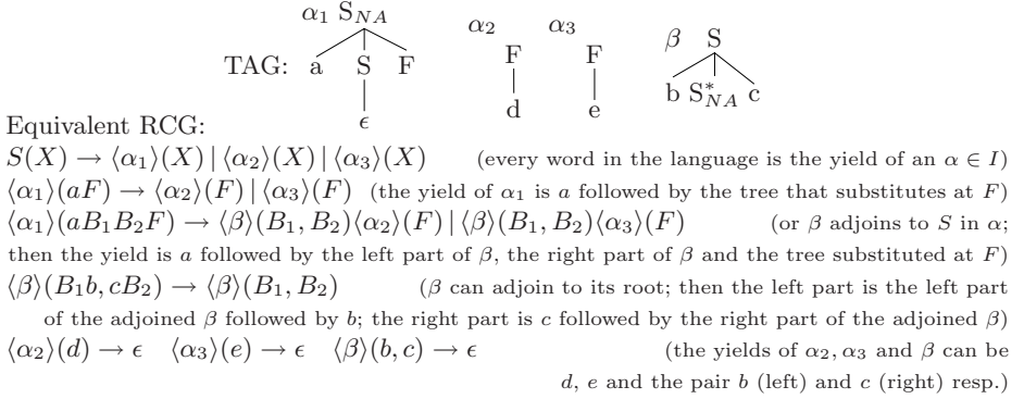
Fig. 2. A sample TAG and an equivalent RCG
