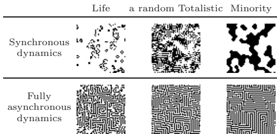
Fig. 2. Typical configurations observed during the evolution of some 2D cellular automata (Moore neighborhood). Similar stripes emerge in asynchronous regime even if their synchronous behavior differ drastically.
