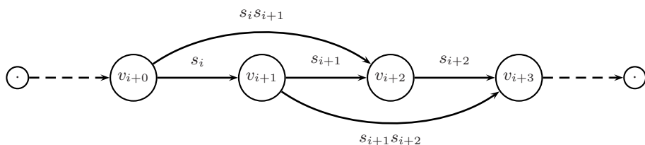
Fig. 1. Graph representation of a phrase
