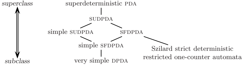
Fig. 1. Related classes of DPDAs to SFDPDAs
