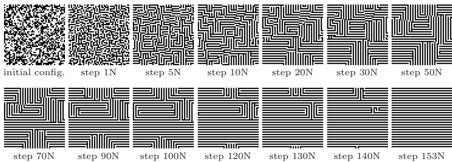
Fig. 3. A typical execution of stochastic 2D Moore minority with N = 50 \times 50 cells
