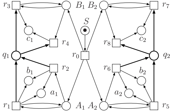
Fig. 3. A 2-PN N_2
