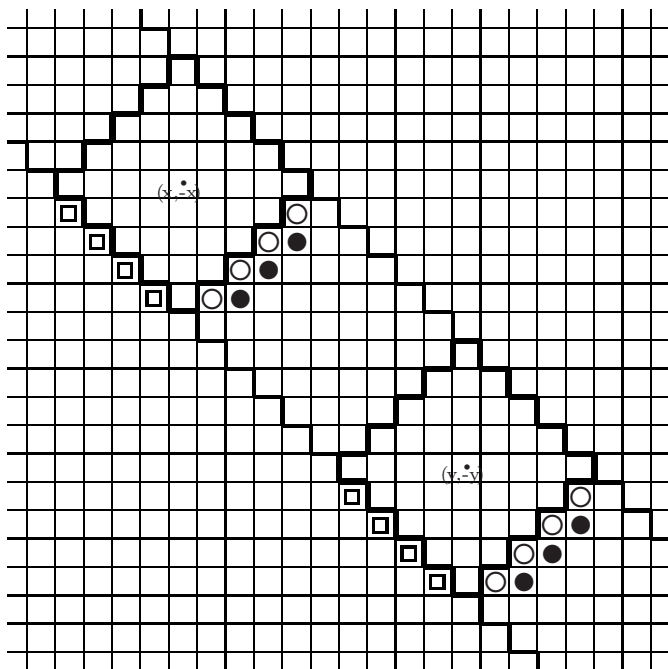
Fig. 4. The illustration for the proof of Proposition 2: the region (z_1, z_2) : |z_1 + z_2| \leq R and two balls B_R(x, -x) and B_R(y, -y) . White circles mark S^1_{R+1}(x, -x) and S^1_{R+1}(y, -y) , black circles mark S^1_R(x + 1, -x - 1) and S^1_R(y + 1, -y - 1) , squares mark the sets S^2_{R+1}(x, -x) and S^2_{R+1}(y, -y) .
