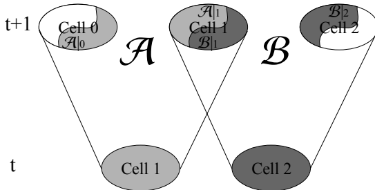
Fig. 1. Definitions of the algebras for the proof of the structure theorem
